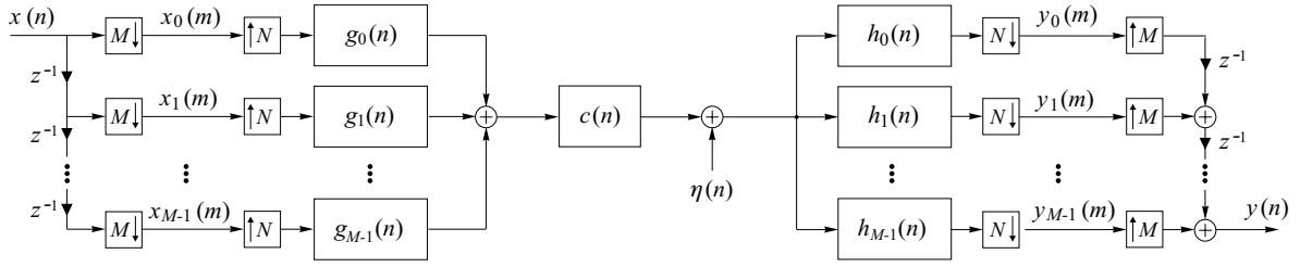
Figure 1: Redundant precoder.
