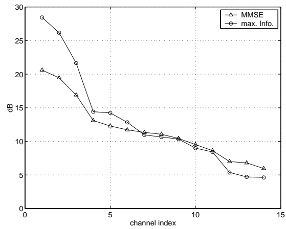
Figure 4: Signal to noise ratios in subchannels at the receiver output.
