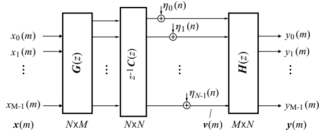
Figure 2: Redundant precoder in polyphase (MIMO) representation.
