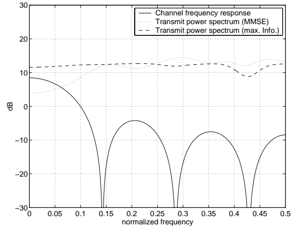
Figure 3: Channel frequency response and transmit power spectra.
