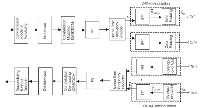
Fig. 1. Structural diagram of the proposed STFC MB-OFDM UWB system.
